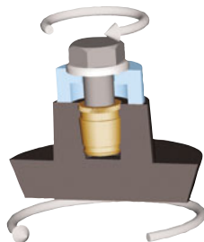
Torque without counter bearing (MA[Nm])**
