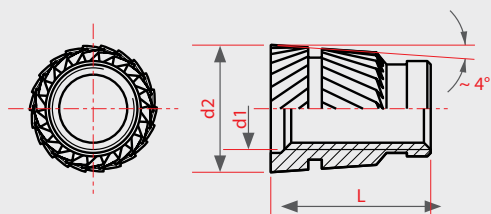
SERIES 853 - 854
