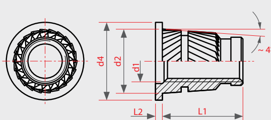
SERIES 855
