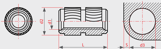
SERIES 863
