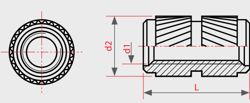
SERIES 864
